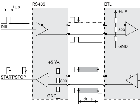
RS-485 signal transmission with digital outputs
