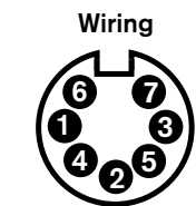
Male insert sensor plug rear or cable connector
